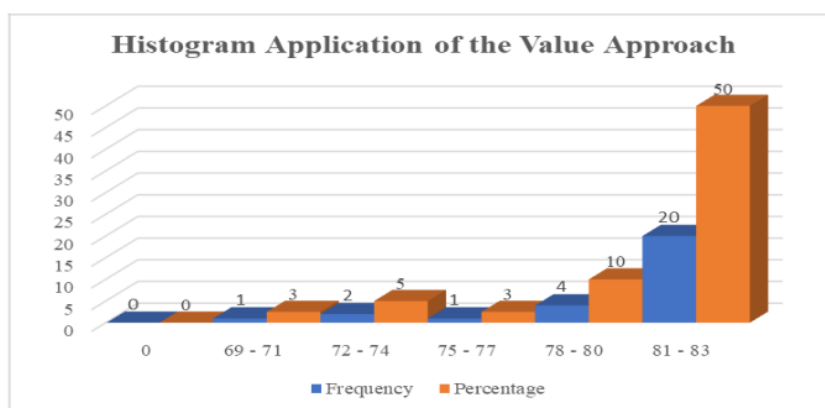
Figure 1. Histogram Application of the Value Approach
