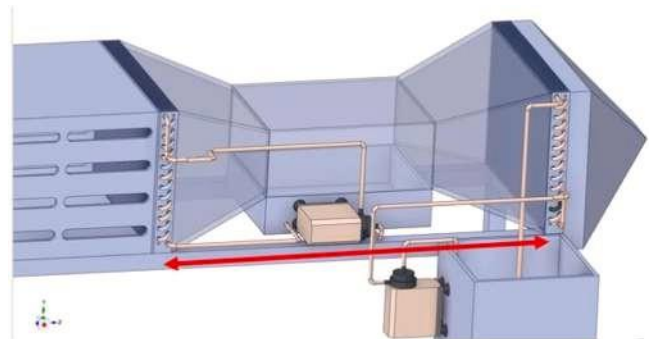
Fig. 1. Simulation model.
