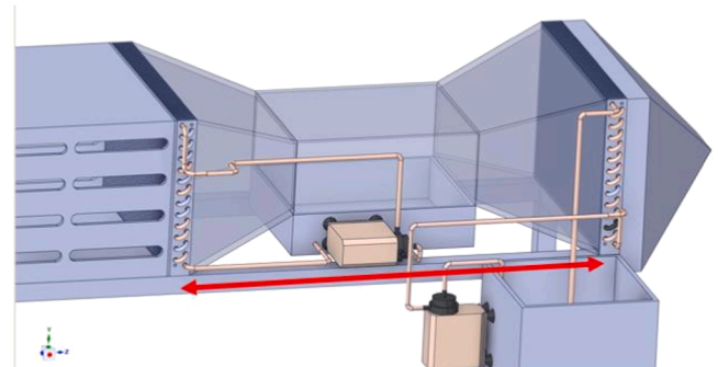
Fig. 1. Simulation model.
