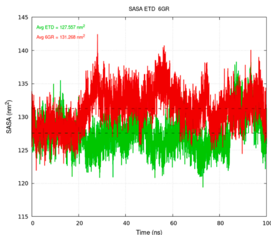
Fig. 19. Compability between ESR1_ETD (green) and ESR1_6 gingerol (red) over 100ns (a) RMSD plot comparing the structural stability (b) The RMSF plot shows the flexibility of amino acid residues (c) The SASA plot presents the solvent-accessible surface area.
