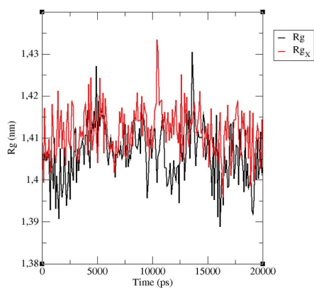
Radius of gyration (total and around axes)
