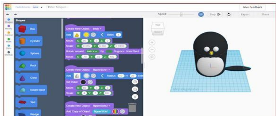
Gambar7.Codeblocks
