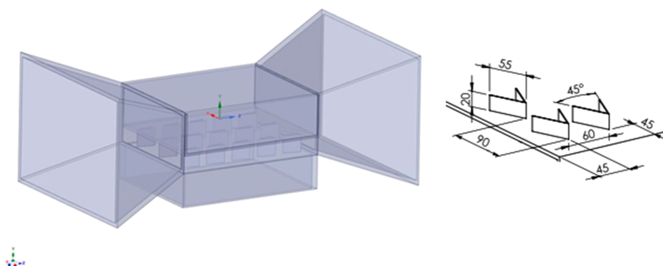
Fig. 2. Simulation variable.
