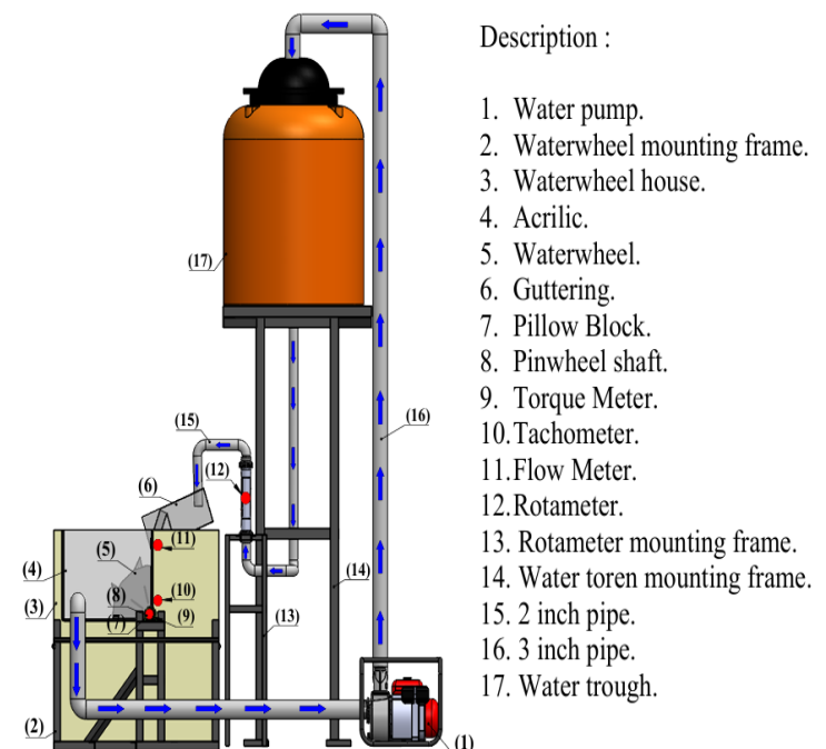
Fig. 4. Schematic design of overshot waterwheel testing installation
