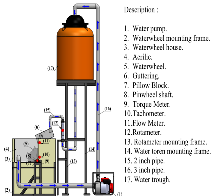
Fig. 4. Schematic design of overshoot waterwheel testing installation
