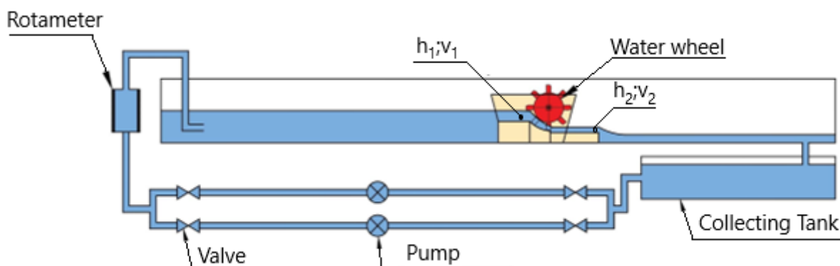
Fig. 4. Experimental setup
