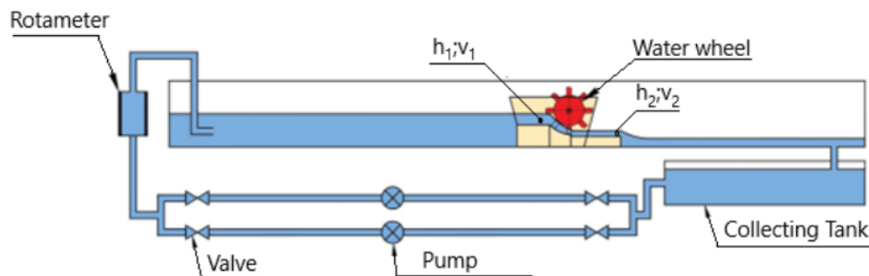
Fig. 4. Experimental setup
