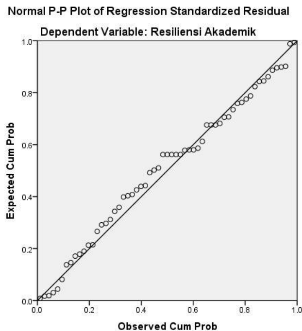
Figure 4 : Probability Graph
