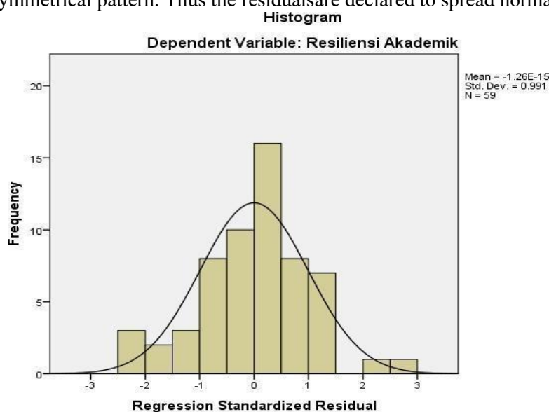
Figure 3 : Histogram
