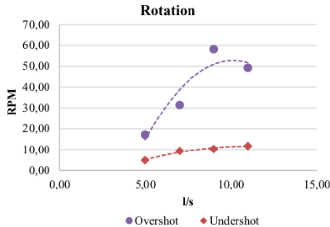
Fig. 2. Rotation of overshoot and undershot dethridge wheel.
