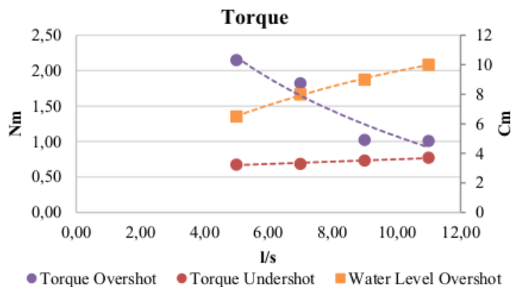
Fig. 3. Torque undershot, overshoot, and water level of overshoot.
