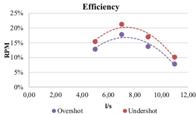
Fig. 6. Efficiency of overshoot and undershot Dethridge wheel.
