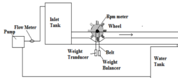
Fig. 1. Schematic of experimental rig.
