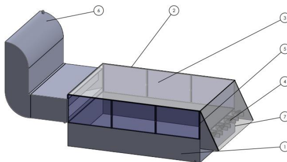
Gambar 1. Alat Desain Penelitian (1) solar still, (2) kaca samping, (3) kaca tetap, (4) akrilik, (5) tiang penyanggah kaca, (6) kondensor, (7) heater
