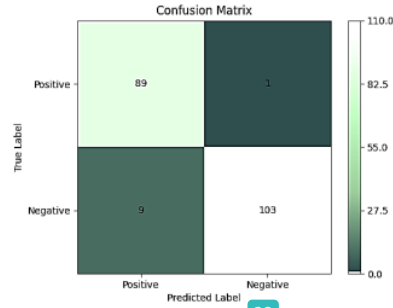
Gambar 9. Visualisasi Confusion Matrix
