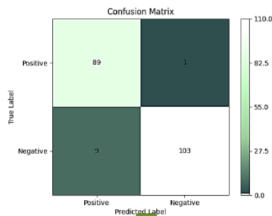
Gambar 7. Confusion Matrix
