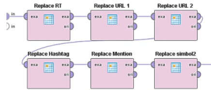
Gambar 4. Cleansing Data
