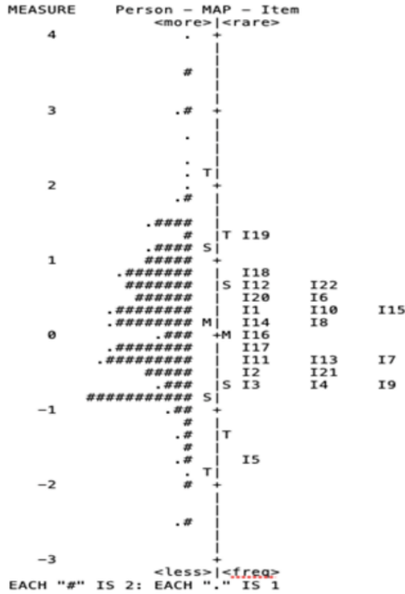
Figure 1 Item-person Wright map
