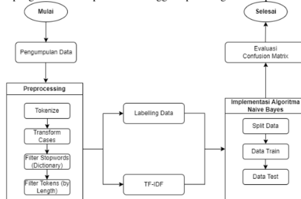
Gambar 1. Alur Penelitian
