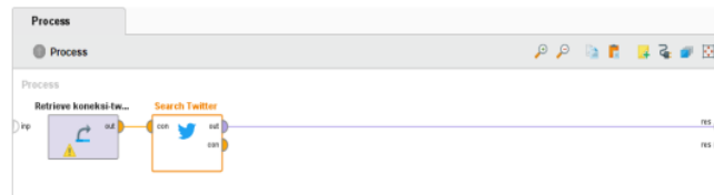
Gambar 3. Crawling Data
