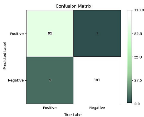
Figure 7. Confusion Matrix Visualization
