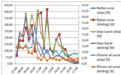
Gambar 1. Distribusi Kinerja Panel Surya (Timur)
