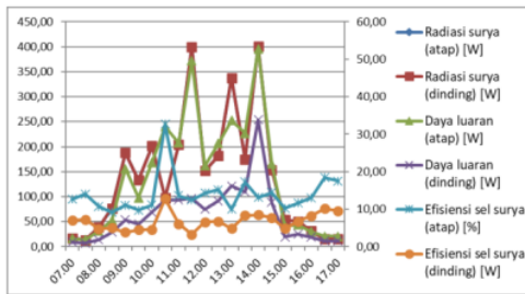
Gambar 3. Distribusi Kinerja Panel Surya (Barat)
