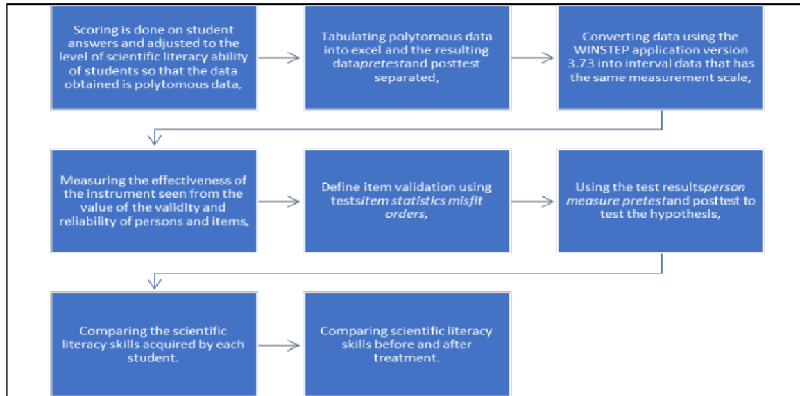
Figure 1. These stages are based on the Rasch model rating analysis approach
