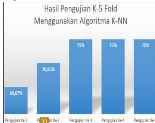
Sumber: ( Malik et al., 2023) Gambar 8. Diagram Chart Pengujian Algoritma K-NN
