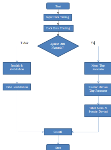
Gambar 3 Flowchart algoritma naive bayes
