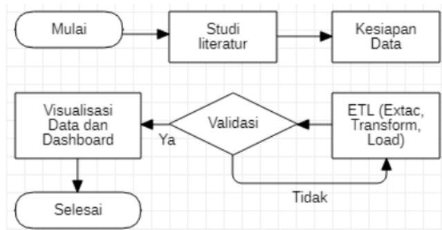
Gambar 1. Flowchart 6 Penelitian
