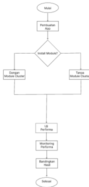
Gambar 1 Alur Proses Clustering
