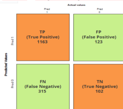
Gambar 9. Tampilan hasil performance vector
