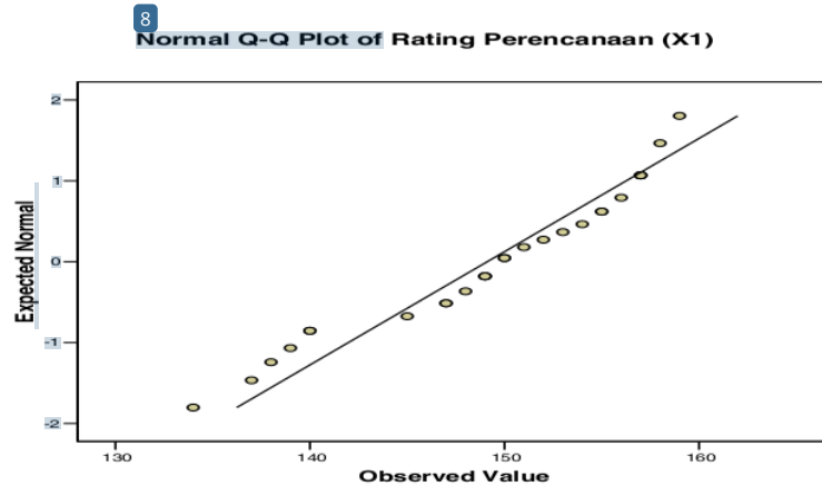
Graphic 1. Data distribution of Variable X1
