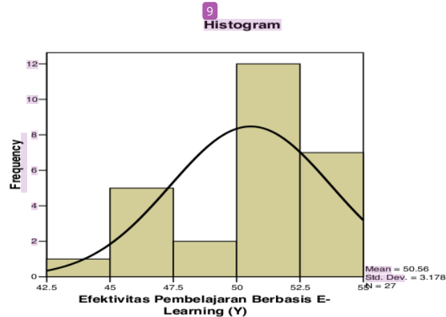
Histogram 4. The Effectiveness of e-Learning (Y)
