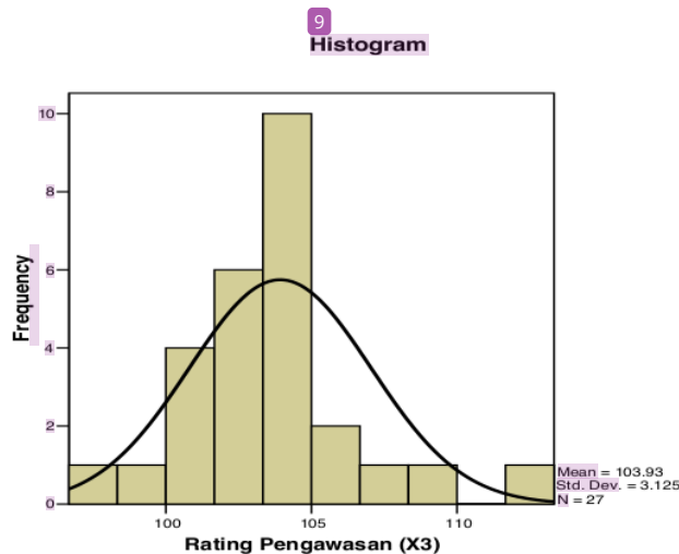
Histogram 3. Rating of controlling (X3)
