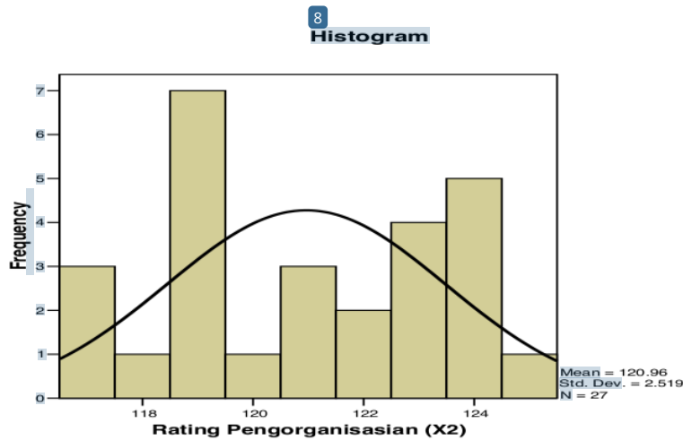
Histogram 2. Rating of organizing (X 2 )
