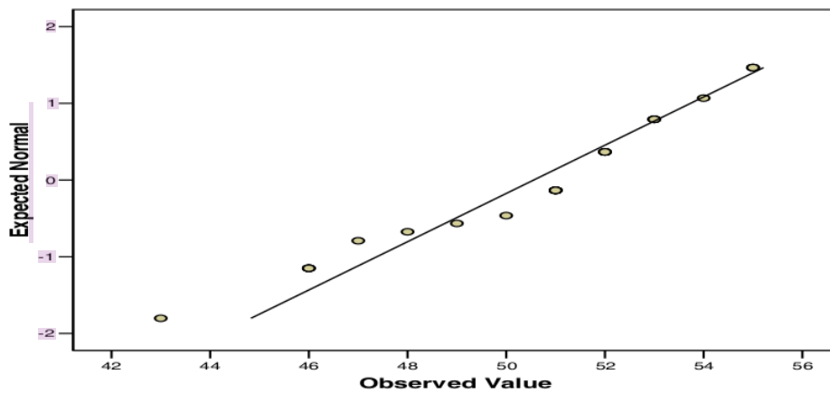
Graphic 4. Data distribution of Variable Y
