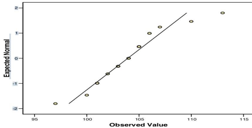
Graphic 3. Data distribution of Variable X3
