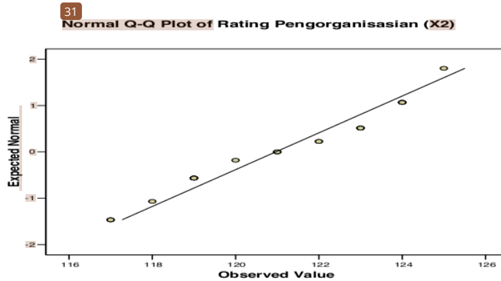
Graphic 2. Data distribution of Variable X2
