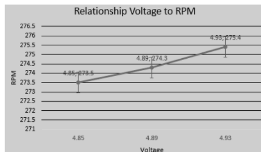
Figure 6. Graph of RPM Against Voltage
