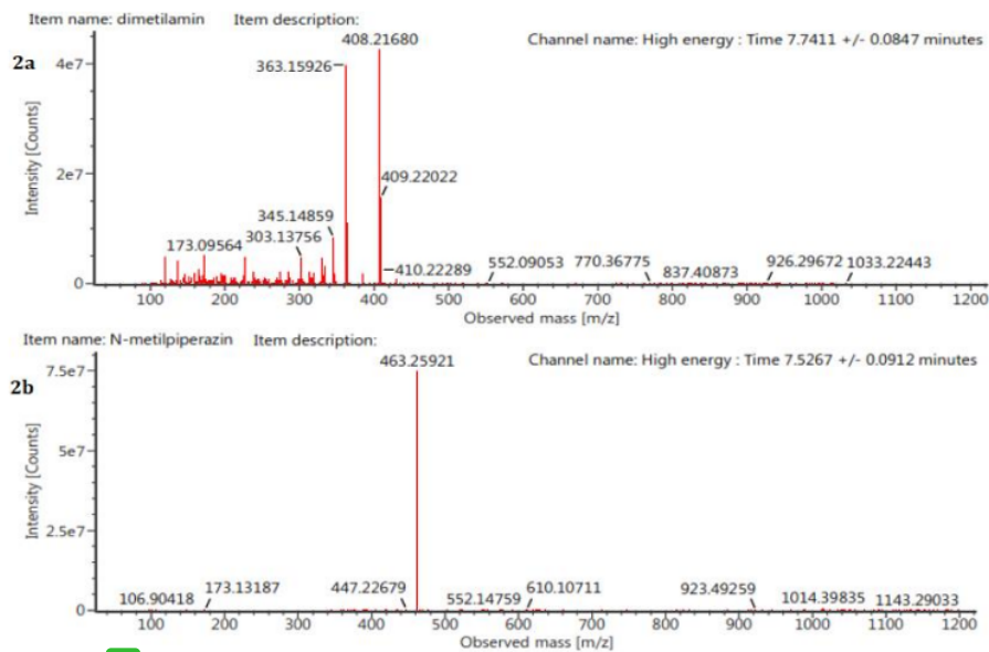
17 Figure 6. Mass spectrum of 2a and 2b
