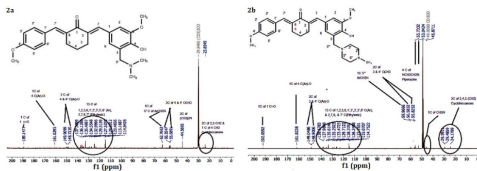
17 Figure 5. 13 C NMR spectrum of 2a and 2b
