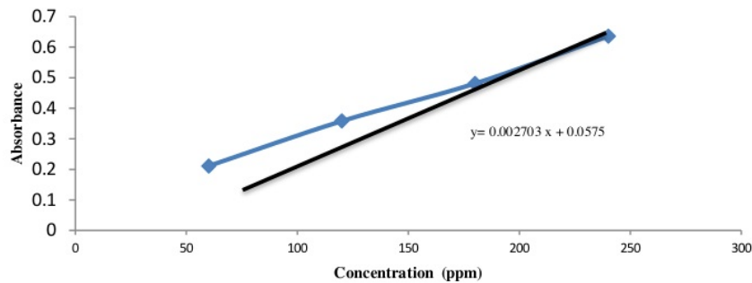
Figure 2: Glutathione in Phosphate buffer pH 6.00 \pm 0.05 .
