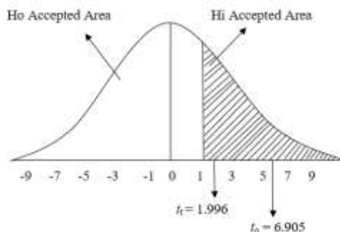
Figure 1. The curve of t-test results
