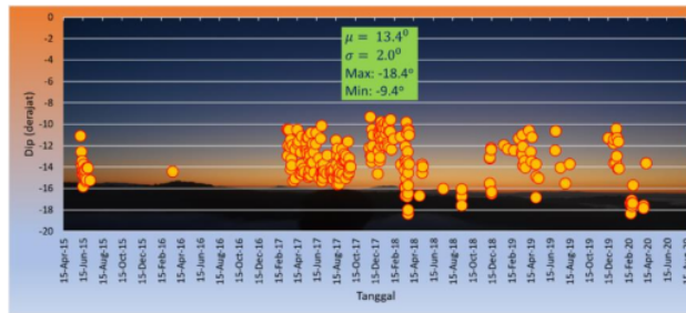
Figure 4: Statistics of the calculated dip from 257 data for the Fajr in Nusantara
