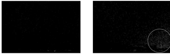
Figure 1: White spots in the white circle (right) verify the presence of the SQM Fajr (Edge detection of image at 4:33:27 (left) and at 5:06:17 (right) in District of Panguk, Province of Yogyakarta, INDONESIA May 12, 2018)
