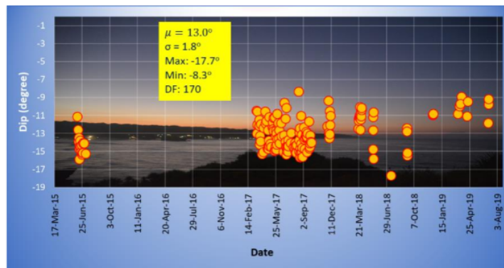
Figure 5: Statistics of the calculated dip from 171 data for the Isha'
