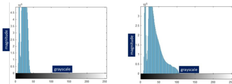
Figure 2: Distinctive difference between the histograms of images at 4:20:50 (left) and 4:41:00 to confirm the presence of the real Fajr according to the SQM data at 4:40:10
