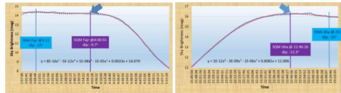
Figure 1: The official and real Fajr in Tacoma on June 18, 2019 (left), real and official Isha in Tacoma on Jun 17, 2019 (right).
