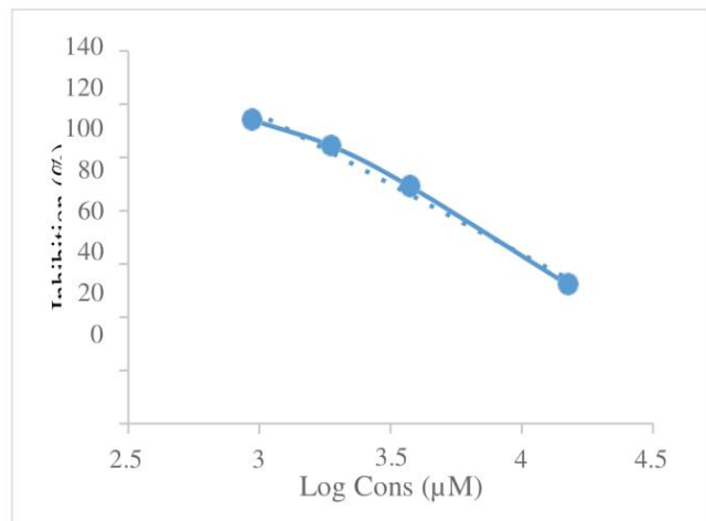
Figure 2. \delta -3-carene Lipoxygenase Inhibition
