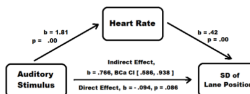
Fig. 9. Model of auditory stimulus as a predictor of SDLP, mediated by heart rate
