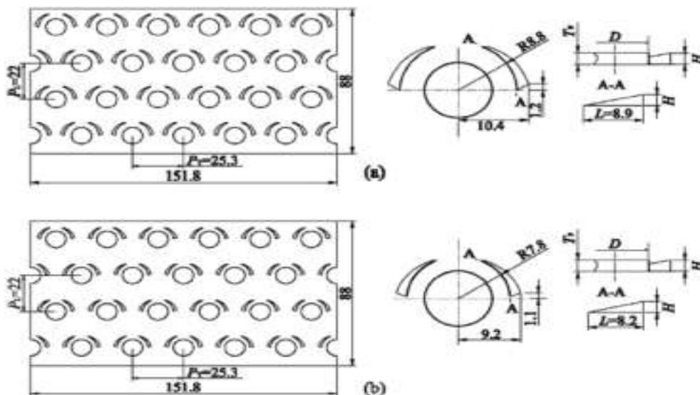
Gambar 4. Geometri curved delta winglet
