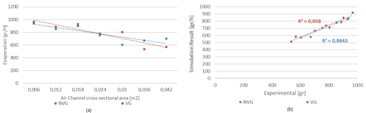
Fig. 5. Evaporation results for each channel cross-sectional area (a) and comparison of the experimental and simulation results (b)
