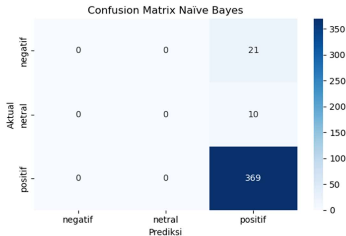
Gambar 14. Confusion Matrix Naïve Bayes
