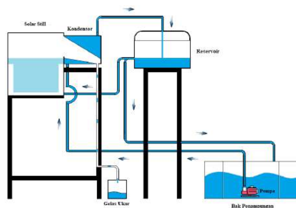
Gambar 1 Skema solar still terpadu
