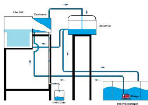
Gambar 1 Skema solar still terpadu
