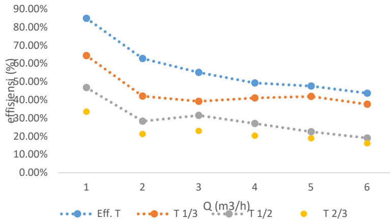
Figure 5. Efficiency Graph
