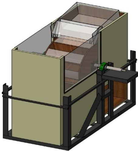
Figure 2. Overall water wheel design
