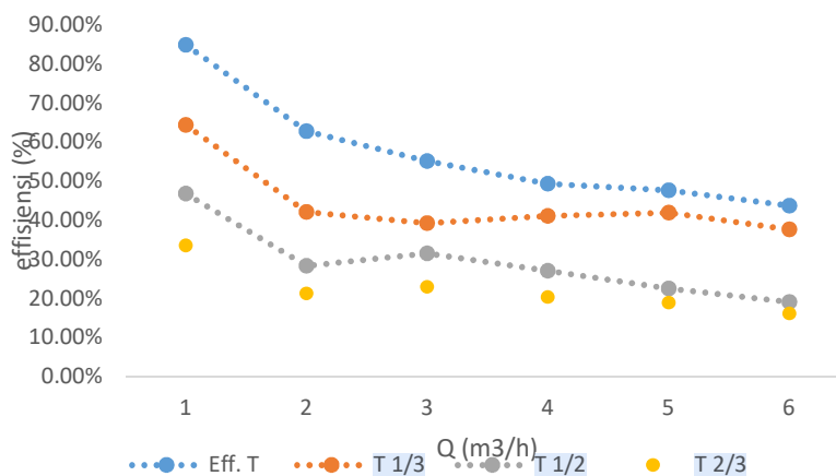
Figure 5. Efficiency Graph
