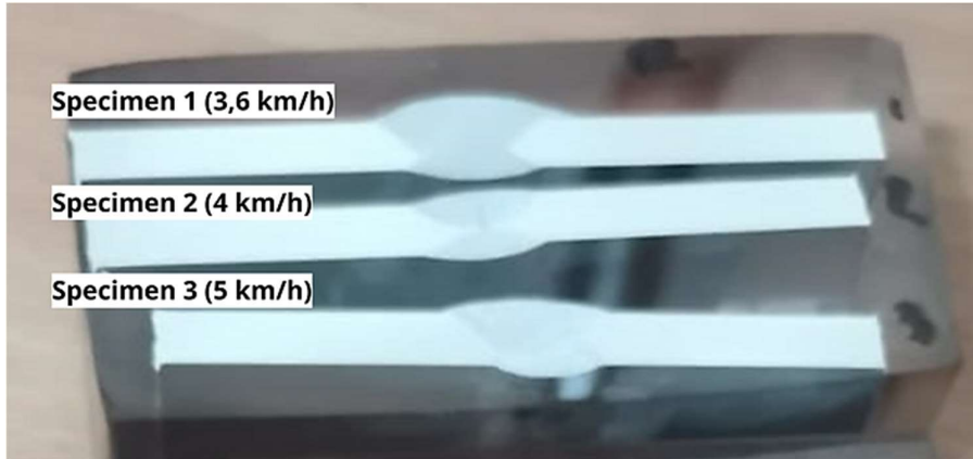
Figure 3. Preparation of vickers hardness testing specimens
