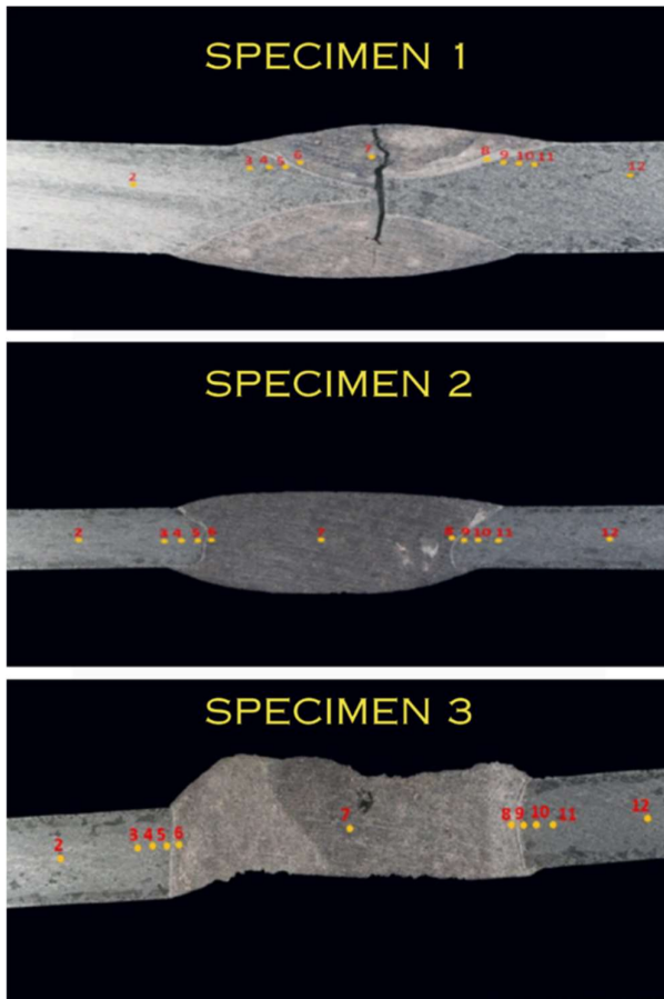
Figure 4. Vickers hardness testing results
