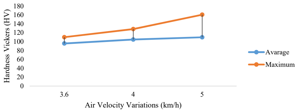
Figure 5. Graph of relation between hardness value and air velocity variation
