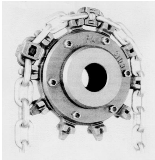
Gambar 2. Rantai Bulat
