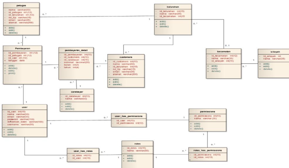
Gambar 4. Class diagram
