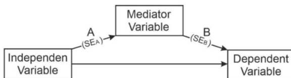
Figure 2 Formula of Sobel Test Analysis
