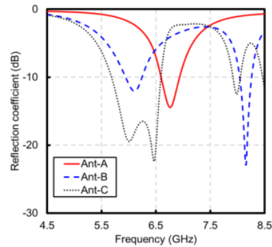
Fig. 2. Reflection coefficient for transformation antenna design.
