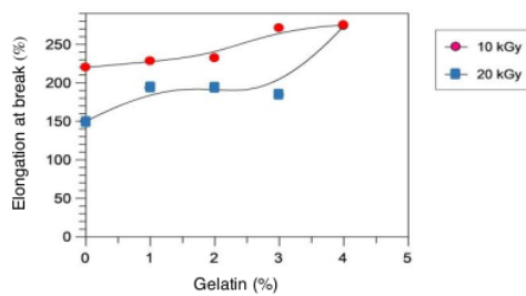
Fig. 6. Effect of gelatin concentration and variation of irradiation dose on the elongation at break of the 10 kGy and 20 kGy PVA-gelatin hydrogels.
