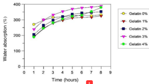
Fig. 3. Relationship between immersion time and water absorption of PVA gelatin hydrogel at irradiation dose of 20 kGy.
