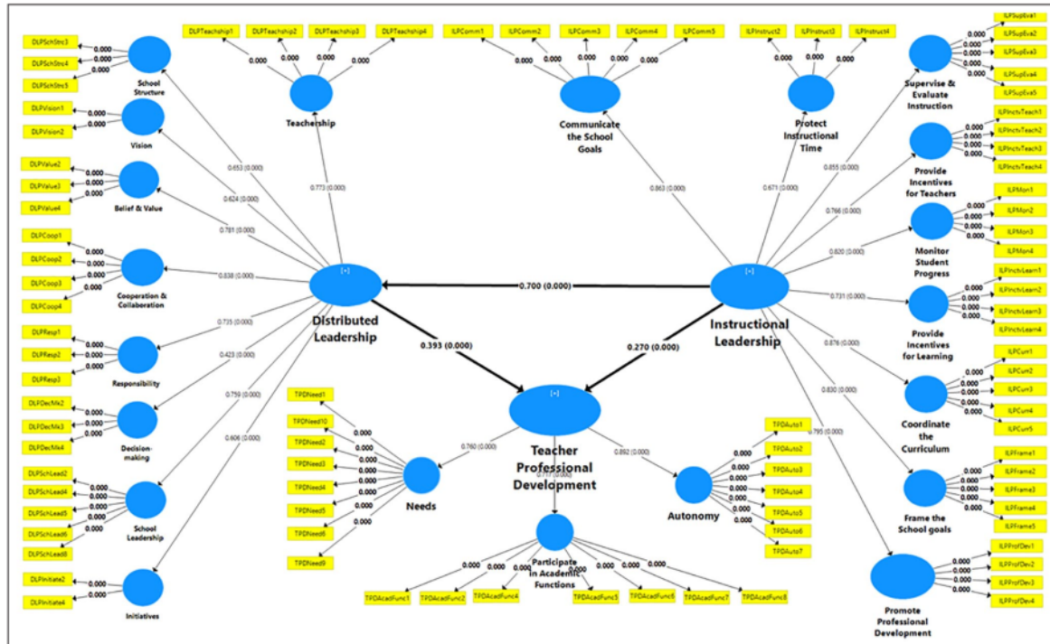
Figure 3. Assessing structural model and path coefficient.
