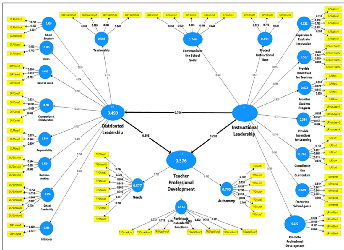
Figure 2. Outer loadings for measurement model.
