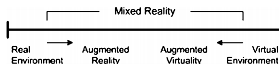
Gambar 1 Reality-Virtual continuum
