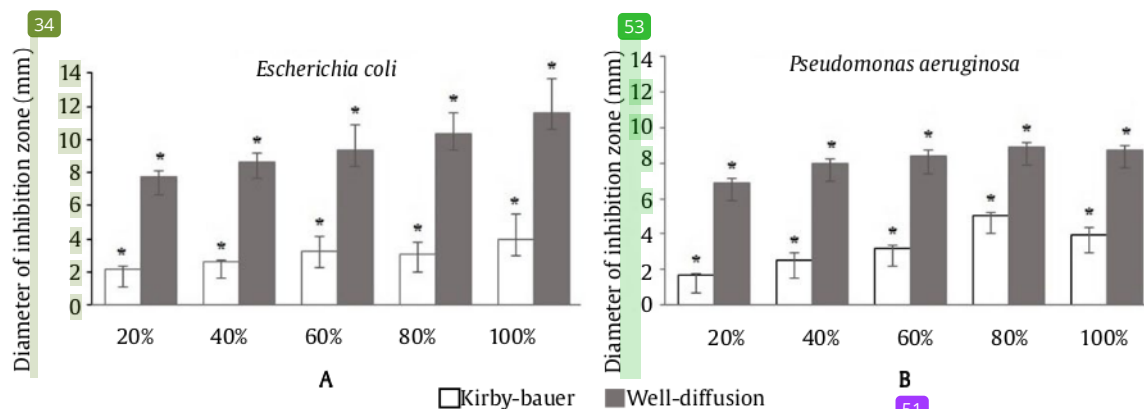
Figure 2. The average diameter of the Kirby-Bauer and well diffusion methods (expressed in diameter of inhibition zone (mm)) produced by (A) Escherichia coli (B) Pseudomonas aeruginosa . *The mean difference is significant at 0.05
