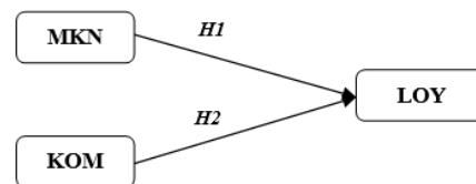
Fig. 1. Research model.
